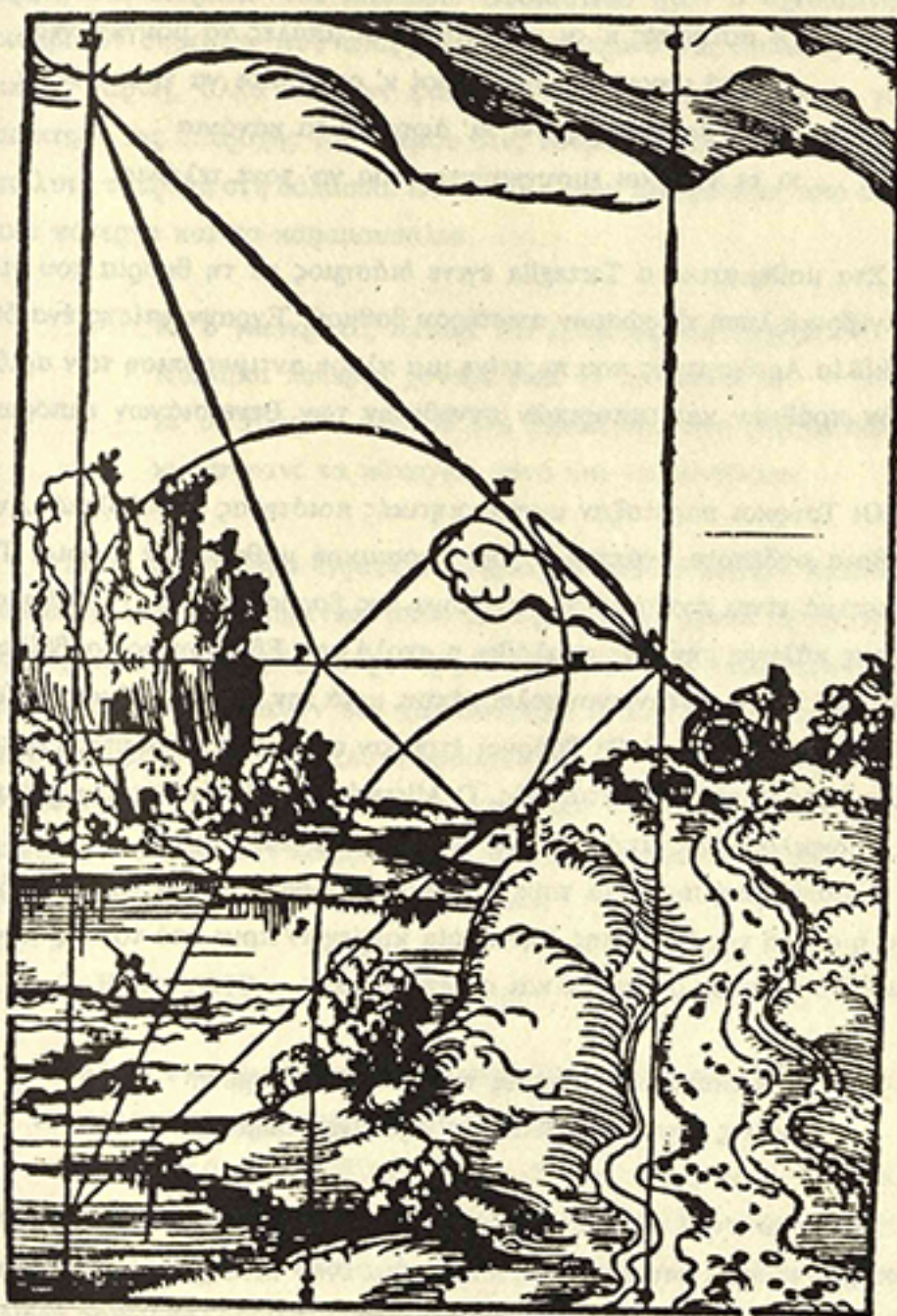
Tartaglia's model of a cannonball's path (sixteenth century)
